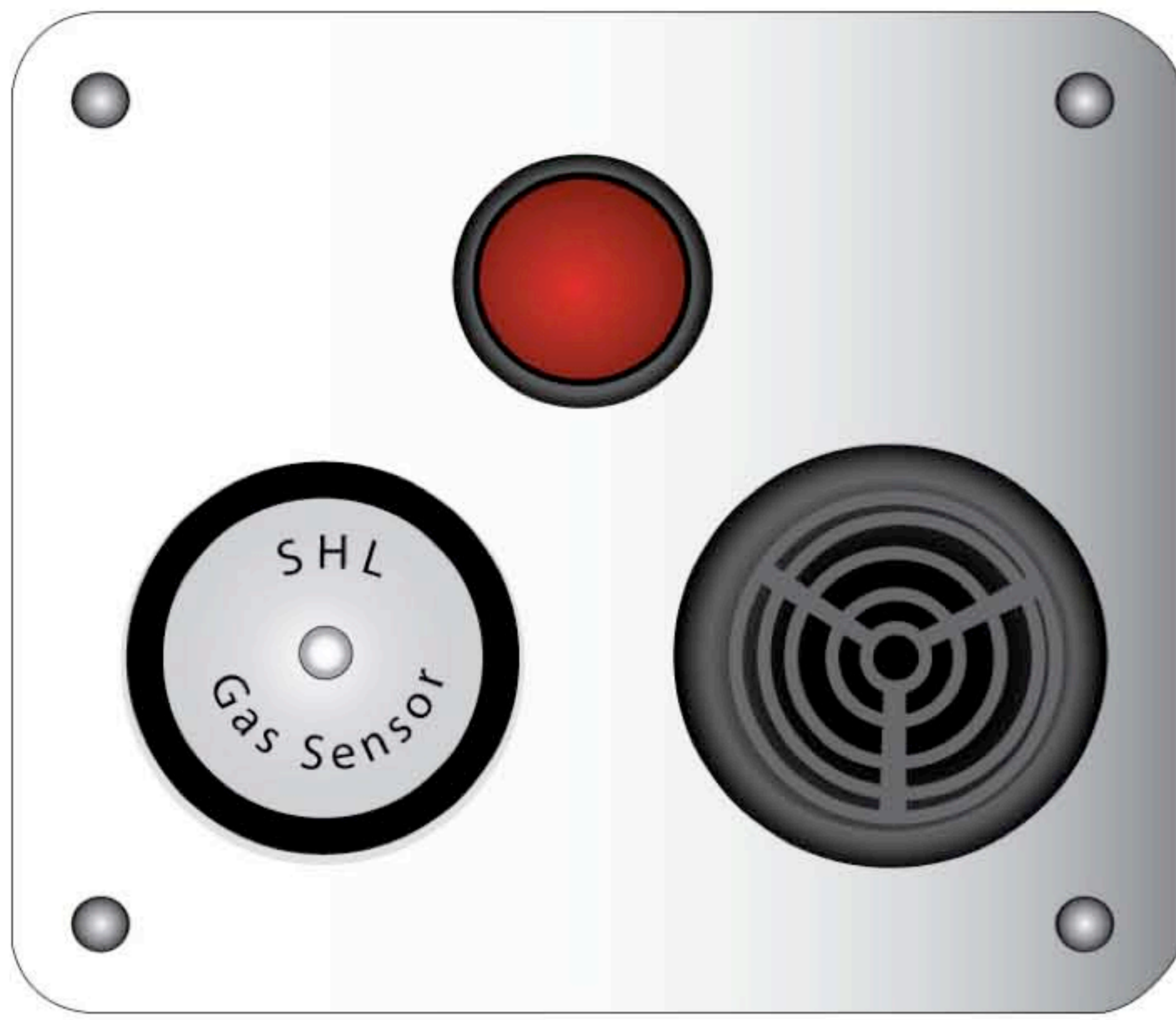
SHL-204 Panel 3.5"L X 3.0"W or 4.375"L X 2.75" W : Gas Sensor LED Red Audible 85 DB LED Red
